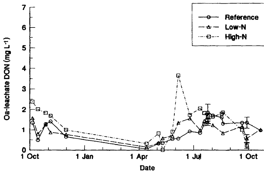
Figure 2. Concentrations of dissolved organic nitrogen (DON) in lysimeter samples from the Oa horizon collected from 5 October 1993 to 21 October 1994. Treatment plots, replication and error bars are as in Figure 1. A. Red pine stand. B. Hardwood stand.
