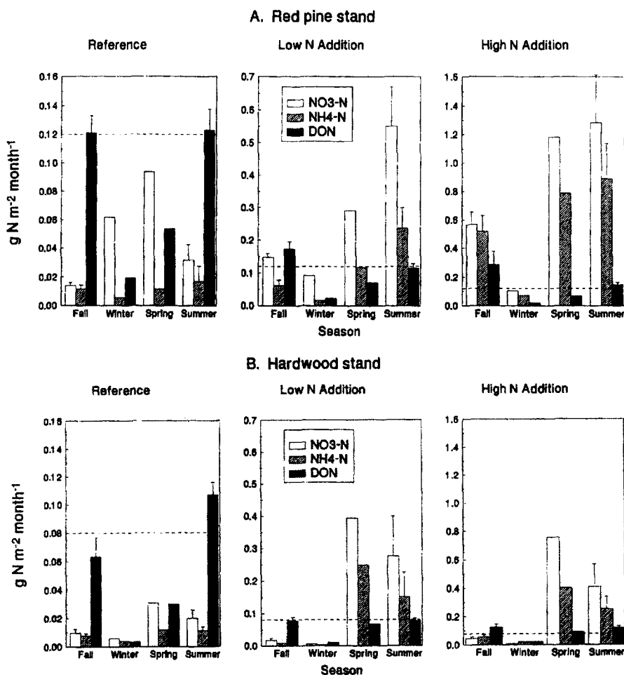
Figure 4. Seasonal fluxes of N eluviated from the Oa horizon. Error bars represent fluxes arising from standard errors of mean concentrations (absent from winter and spring fluxes because snowmelt was sampled only on one date). Note the extreme differences in scale among plots within each stand: reference lines are provided to facilitate direct comparison among reference and N addition plots. A. Red pine stand. B. Hardwood stand.
