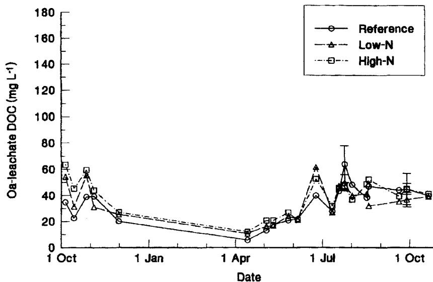
Figure 1. Concentrations of dissolved organic carbon (DOC) in lysimeter samples from the Oa horizon collected from 5 October 1993 to 21 October 1994. Results from reference, low-N addition and high-N addition plots are shown. Values indicated represent chemistry of bulked samples from 5 replicate collections within each treatment. Error bars represent standard errors from the two dates on which samples remained unbulk for analysis. A. Red pine stand. B. Hardwood stand.
